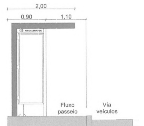
V. Vista
